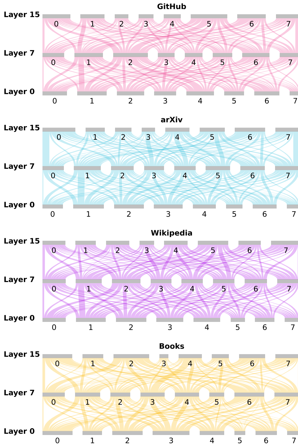
Figure 36: Mixtral-8x7B token routing across layers. We visualize how often tokens from different domains get routed to a pair of experts across layers under top-1 routing, corresponding to Figure 34 . The size of each rectangle is proportional to the total number of tokens an expert receives, while the flow between two experts shows the proportion of tokens routed to both experts. The flows between layers 0 → 7 and 7 → 15 are independent in this visualization.
