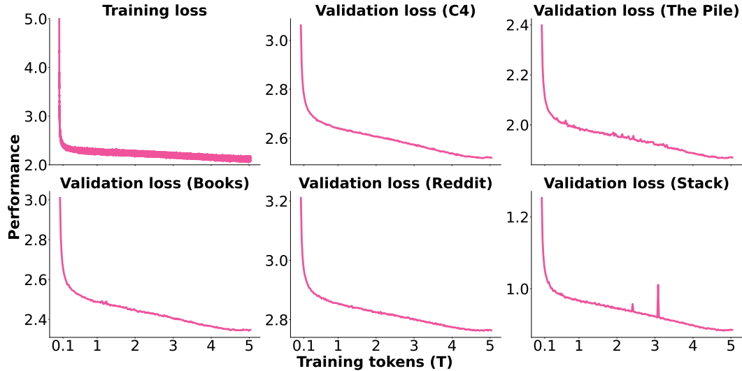
Figure 24: Losses of OLMoE-1B-7B during training. The Books, Reddit, and Stack [83] datasets are from Dolma 1.7 [161] via Paloma [110]. More results, logs, and configurations: https://wandb.ai/ai2-llm/olmoe/reports/Plot-OLMoE-1B-7B--Vml1dzo40TcyMjU3
