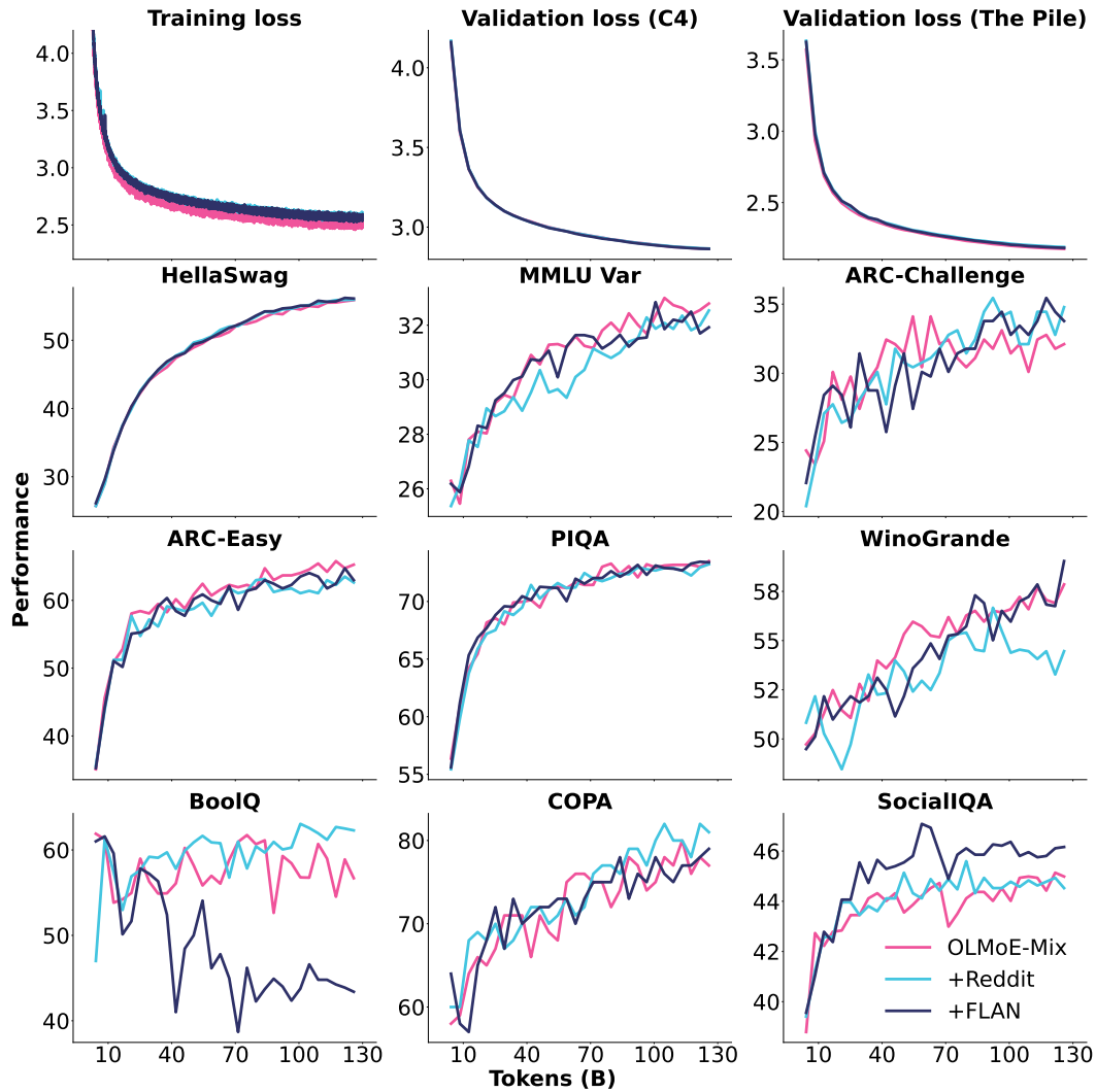
Figure 26: Adding Reddit or FLAN to OLMoE-Mix. More results, logs, and configurations: https://wandb.ai/ai2-llm/olmoe/reports/Plot-Adding-Reddit-FLAN--Vml1dzo40Tg1NTg4
