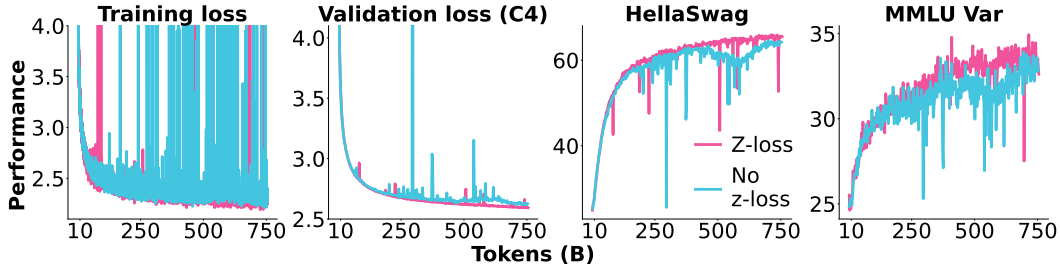
Figure 11: Router z-loss . We compare adding router z-loss with a loss weight of 0.001 versus no additional z-loss. More results, logs, and configurations: https://wandb.ai/ai2-llm/olmo/reports/Plot-Zloss-vs-none--Vmlldzo4NDM4NjUz
