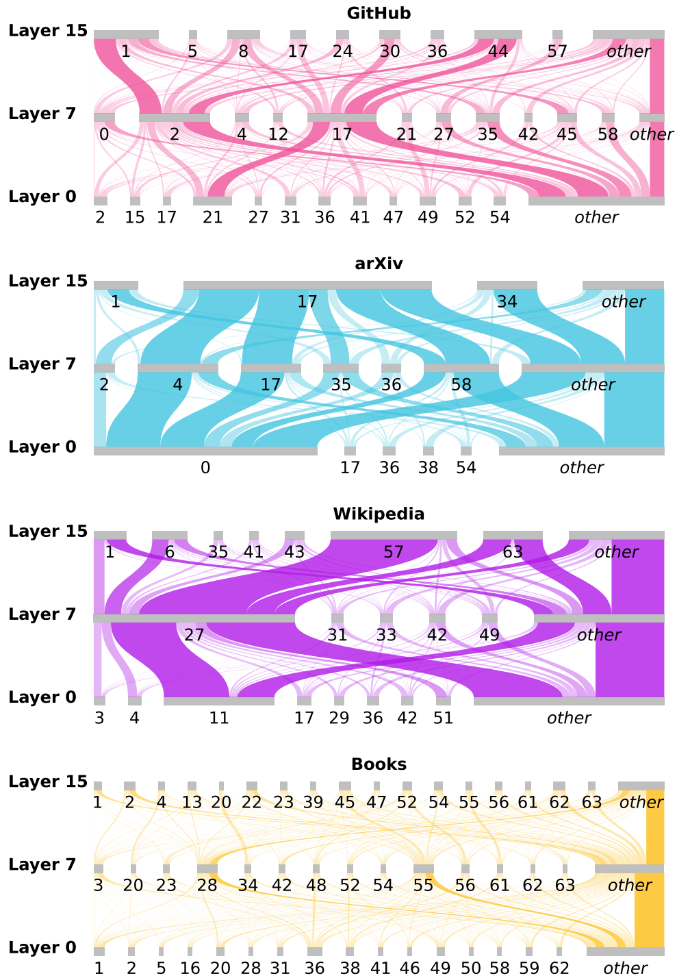
Figure 35: OLMoE-1B-7B token routing across layers. We visualize how often tokens from different domains get routed to a pair of experts across layers under top-1 routing, corresponding to Figure 34. The size of each rectangle is proportional to the total number of tokens an expert receives, while the flow between two experts shows the proportion of tokens routed to both experts. We only show experts that receive tokens 50% above random chance and use stronger coloring for larger flows. We observe some instances of cross-layer coordination between pairs of experts, e.g., expert 27 in layer 7 and expert 57 in layer 15 process a substantial fraction of Wikipedia tokens together. The flows between layers 0 \rightarrow 7 and 7 \rightarrow 15 are independent in this visualization.
