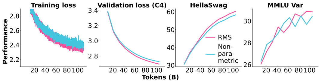
Figure 14: Non-parametric layer normalization vs. RMSNorm. More results, logs, and configurations: https://wandb.ai/ai2-llm/olmoe/reports/Plot-LN--Vml1dzo4NDQyMTAz
