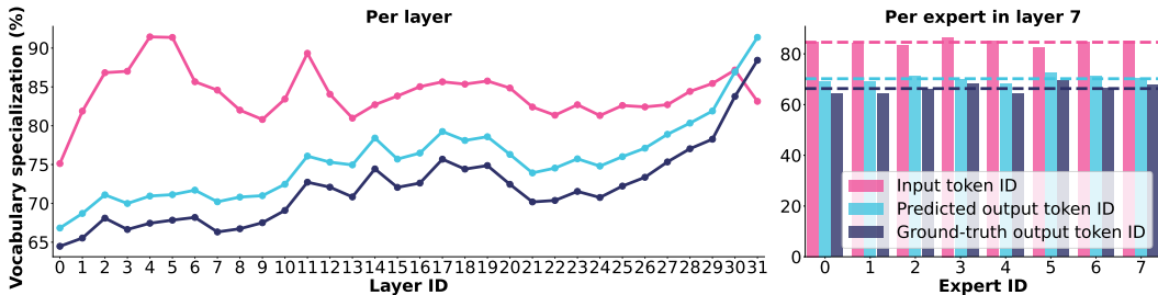
Figure 31: Vocabulary specialization for Mixtral-8x7B when considering all 2 activated experts. Equivalent to k = 2 in Equation 8.
