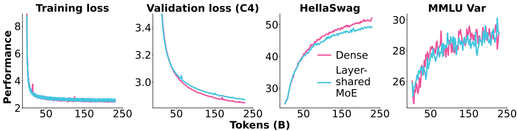
Figure 29: Sharing the same MoE across layers versus a regular dense LM. The number of experts in the MoE is equivalent to its number of layers. Thus, because the MoE is shared across layers, it has the same number of total and active parameters as the dense model. More results, logs, and configurations: https://wandb.ai/ai2-llm/olmoe/reports/Plot-Shared-vs-Dense--Vmlldzo4NDIOMTc5
