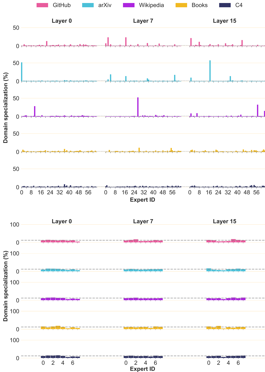
Figure 34: Domain specialization of OLMoE-1B-7B (top) vs. Mixtral-8x7B (bottom) of the top-1 routed expert. We visualize how often tokens from different domains get routed to the 64 (OLMoE) or 8 (Mixtral) experts at the end of pretraining. Unlike in Figure 22, here we only consider tokens routed to the top-1 expert ( k = 1 in Equation 7). Horizontal gray lines correspond to uniform routing ( 1/64=1.56\% per expert for OLMoE-1B-7B and 1/8=12.5\% for Mixtral).
