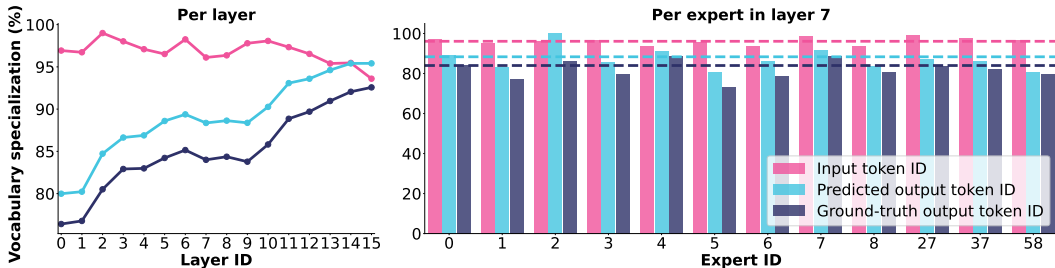
Figure 30: Vocabulary specialization for OLMoE-1B-7B when considering all 8 activated experts. Equivalent to k = 8 in Equation 8.
