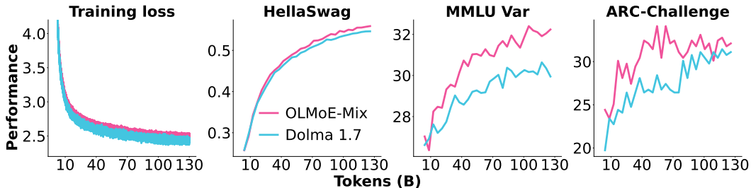
Figure 12: OLMoE-MIX vs. Dolma 1.7 . We compare our data mix described in §2 with Dolma 1.7 used to train prior OLMo models. Lower training loss does not mean that one dataset is better, but rather suggests which dataset is easier for the model to learn. More results, logs, and configurations: https://wandb.ai/ai2-llm/olmo/reports/Plot-Dolma-1-7-vs-Dolma-OLMoE--Vmlldzo40TixNTg5
