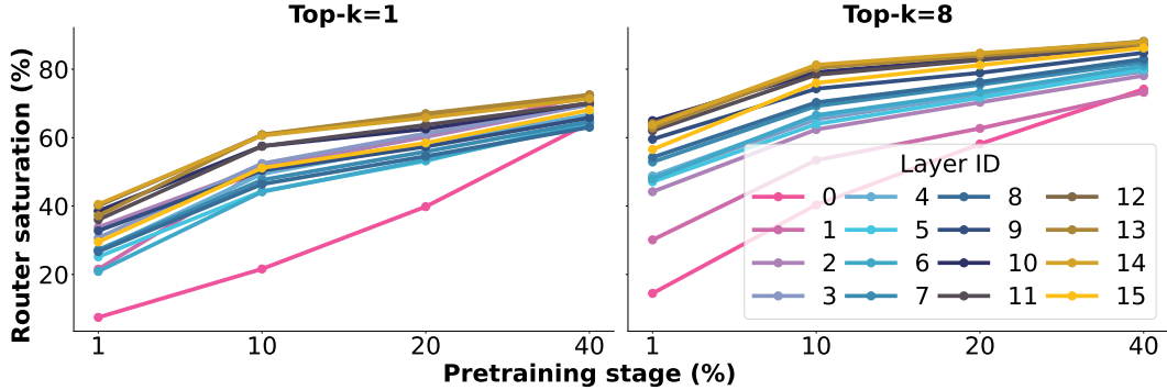
Figure 20: Router saturation during pretraining measured on a random 0.5% of the C4 validation data. We compute saturation by comparing the routing to the top- k experts at four intermediate checkpoints (1, 10, 20, and 40% of pretraining) to the final pretraining checkpoint (Equation 5).
