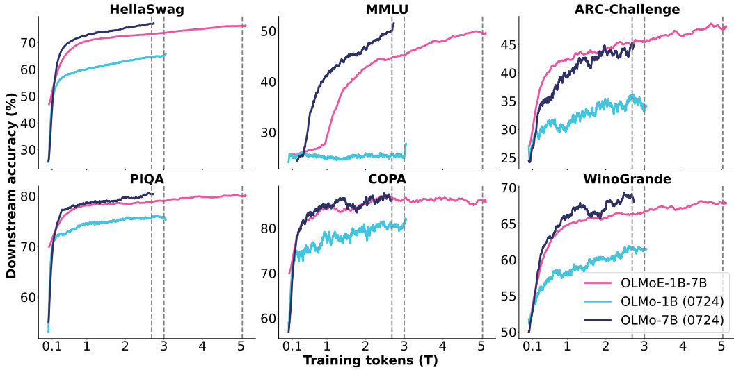
Figure 25: Evaluation of OLMoE-1B-7B and the current best OLMo models during pretraining. Grey vertical lines correspond to where the respective run enters annealing with the 1st line being for OLMo-7B, the 2nd for OLMo-1B, and the third for OLMoE-1B-7B . Figure 3 is a version of this plot with training FLOPs as the x-axis. More results, logs, and configurations: https://wandb.ai/ai2-llm/olmoe/reports/Plot-OLMoE-1B-7B-vs-OLMo-7B-vs-OLMo-1B--Vmlldzo40TcyMjEz
