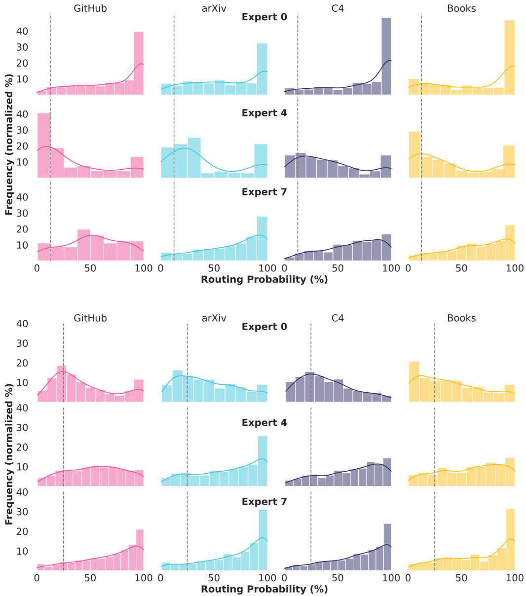
Figure 32: Vocabulary specialization across domains of OLMoE-1B-7B (top) and Mixtral-8x7B (bottom). We visualize how often token IDs get routed to specific experts. We only include IDs that appear at least 8 times in the various corpora. Vertical gray lines correspond to uniform routing ( 8/64=12.5\% for OLMoE-1B-7B as it has 64 experts, 8 of which are activated; 2/8=25\% for Mixtral as it has 8 experts, 2 of which are activated). For example, among all token IDs in GitHub that get routed to Expert 0 at least 8 times for OLMoE-1B-7B, \sim 40\% of them get routed to Expert 0 with a probability of \sim 100\% (upper left) indicating that Expert 0 is specialized on those token IDs. For OLMoE-1B-7B there is much frequency at the routing probability extremes (0% or 100%) indicating that these experts exclusively focus on certain token IDs, especially for specific domains (§5.3) like GitHub and arXiv.
